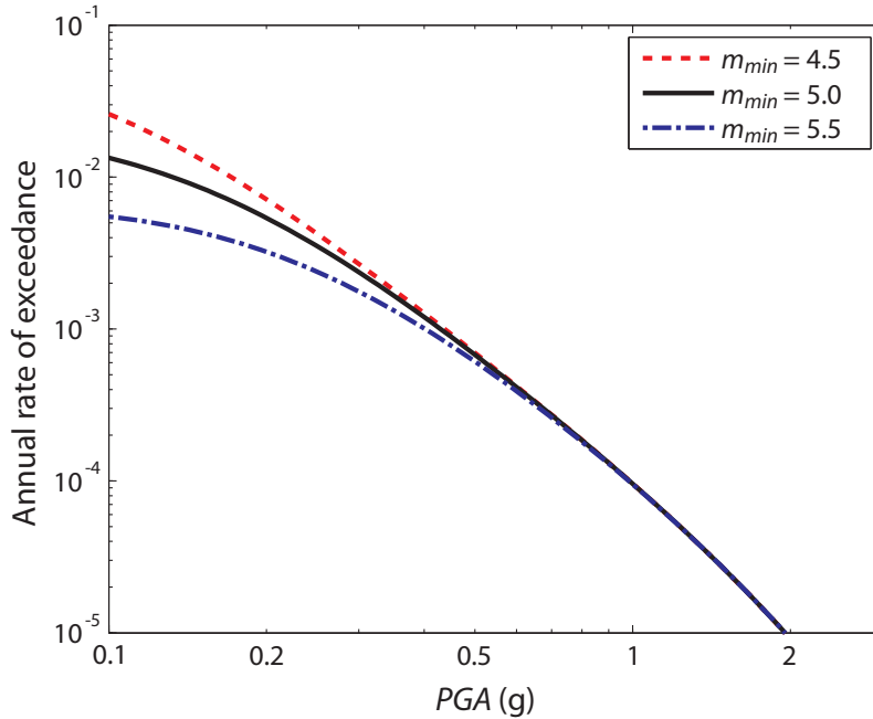
Figure 3.4: Hazard curves computed for the example site from Section 2.4, using several choices for the minimum considered magnitude.
