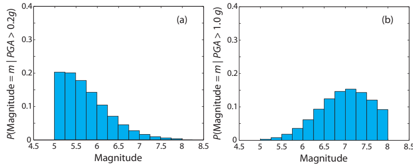
Figure 3.1: Deaggregation results associated with the example calculation of Section 2.4. (a) Magnitude distribution, given PGA > 0.2g . (b) Magnitude distribution, given PGA > 1g .
