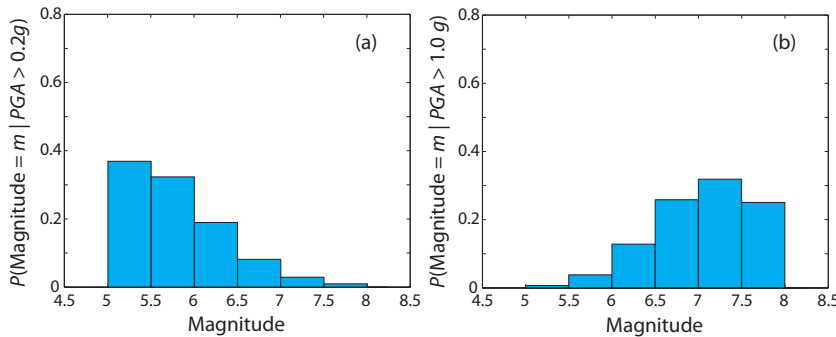
Figure 3.2: Deaggregation results associated with the example calculation of Section 2.4, with magnitudes discretized into 0.5-unit intervals. (a) Magnitude distribution, given PGA > 0.2g . (b) Magnitude distribution, given PGA > 1g .
